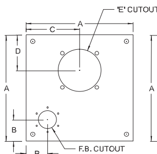
Cover with Filler Breather Cutout and 56C/145TC Adapter Cutout (Adapter Style 1, 1A, 1B) Part Number 99937
