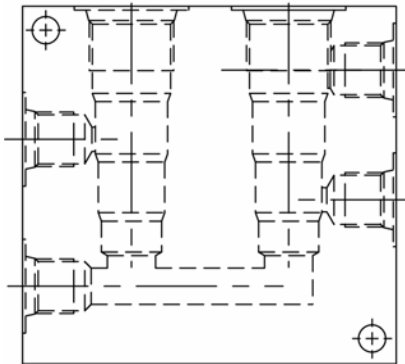
BASE BODY - 20200008 = #6 SAE
