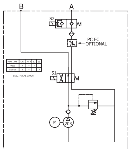
HYDRAULIC SCHEMATIC
