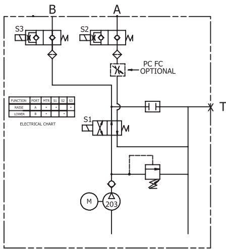
HYDRAULIC SCHEMATIC
