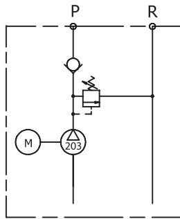
HYDRAULIC SCHEMATIC
